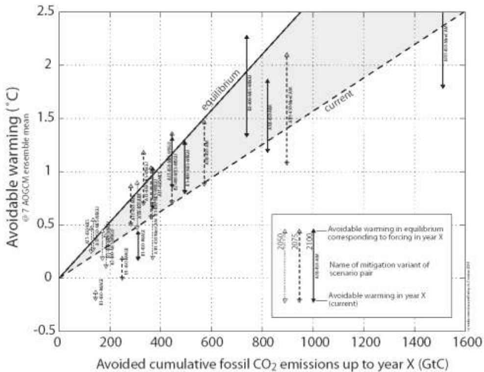
Figure 2 Climate models linking changes on CO 2 emissions to a change in temperature
